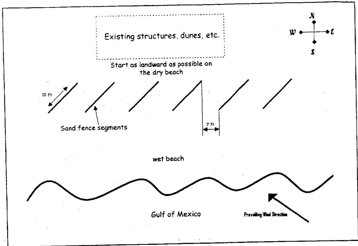
Figure 15. Dune restoration fence alignment.
